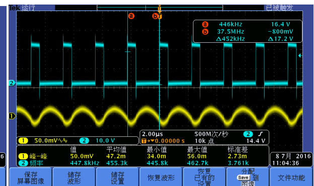
IN:16V,OUT:5V/3A
